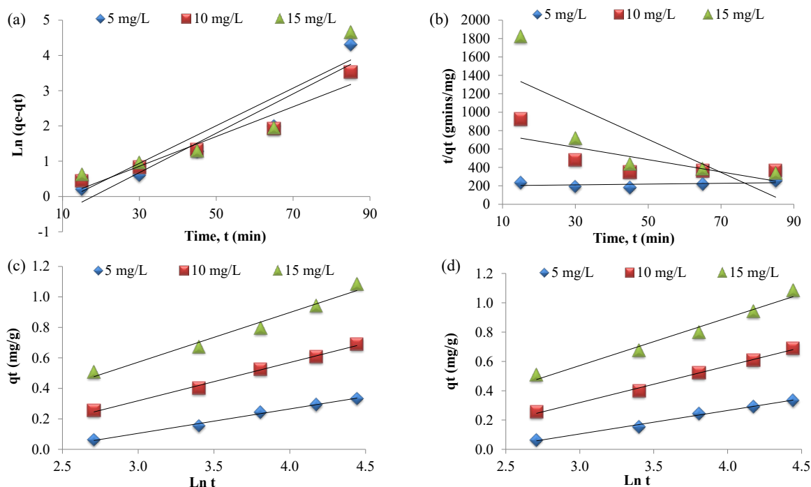
Figure 8 – (a) Pseudo First Order Kinetics Model (b) Pseudo Second Order Kinetics Model (c) Elovich Model (d) Avrami Model for the removal of DCF-Na onto modified BKW composite
