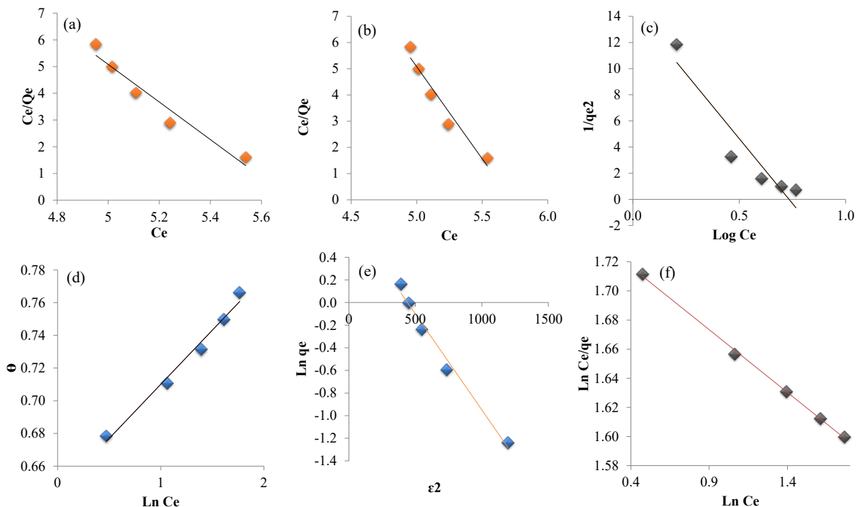
Figure 7 – Adsorption isotherms of 10 mg/l DCF-Na onto 1 g of BKW composite. Fitting of the experimental data to (a) Langmuir (b) Freundlich (c) Harkin-Jura (d) Temkin (e) Dubinin-Radushkevich (f) Redlich-Peterson isotherm models carried out at room temperature (25°C)
