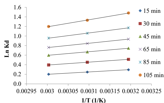
Figure 10 – Vant Hoff's model plot for DCF-Na removal from solution onto modified BKW composite
