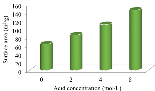
Figure 2 – Variation of surface area of the unmodified (UAM) and modified (2, 4, and 8 mol/L) Kaolin samples
