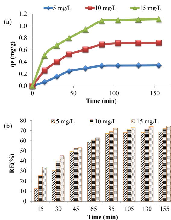
Figure 5 – (a) Adsorption Capacity (b) Removal Efficiency (RE) plot describing the effect of concentration of DCF-Na using 1 g of H 3 PO 4 modified BKW composite (1:2:1) at room temperature
