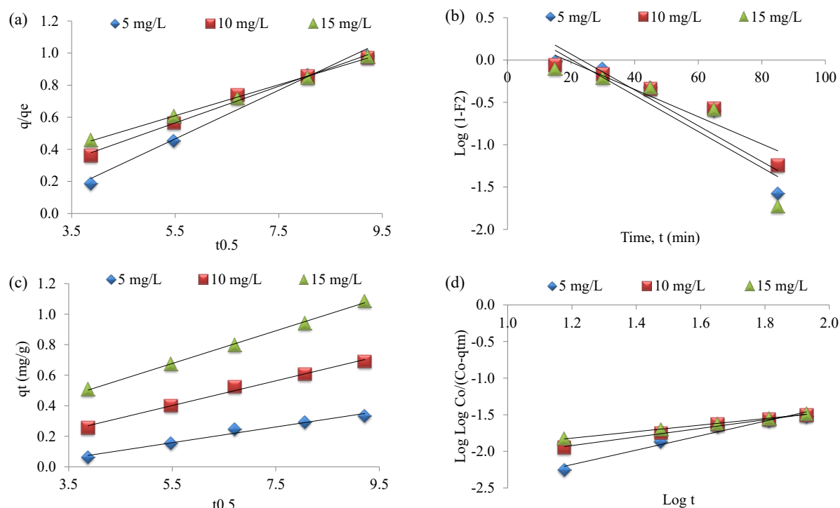
Figure 9 – (a) Crank (b) Vermeulen (c) Weber Morris (d) Banghams diffusion model for the removal of DCF-Na from modified BKW composite
