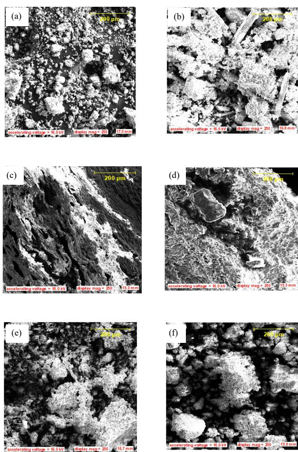
Figure 4 – Scanning Electron Microscopy for modified and unmodified Bentonite (a and b), Kaolin (c and d), and Wormcast (e and f)
