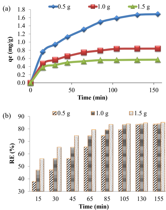
Figure 6 – (a) Adsorption Capacity (b) Removal Efficiency (RE) plot describing the effect of geosorbent dose on the adsorption of 10 mg/L DCF-Na onto H_3PO_4 modified BKW composite (1:2:1) at room temperature
